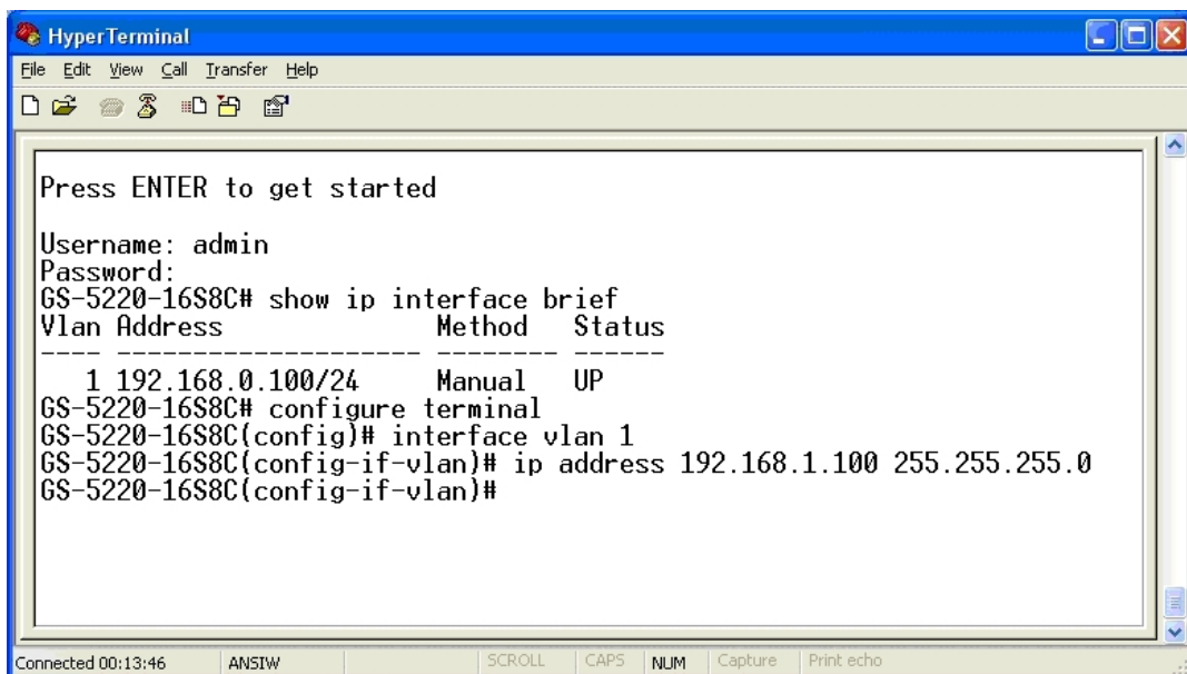
Figure 3-3: Configuring IP Address Screen
