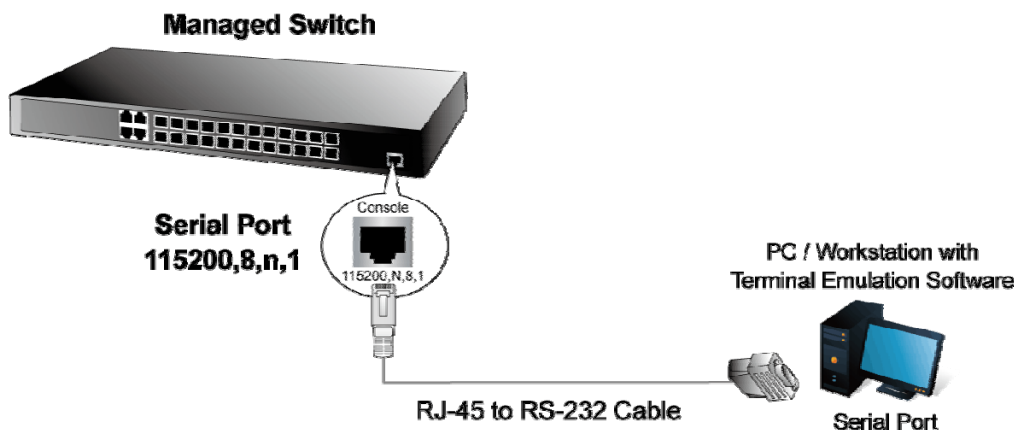
Figure 2-1 Managed Switch Console Connectivity
